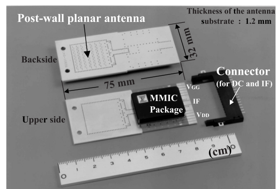
Fig. 1 A cost-effective 60 GHz module with a post-wall planar antenna.
