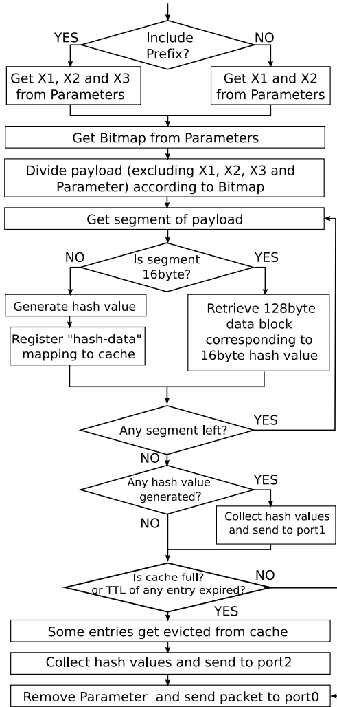
Fig. 8 Flow of operations at egress router.
