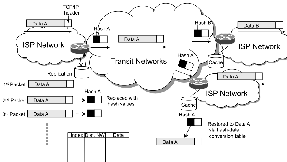
Fig. 1 Design overview.
