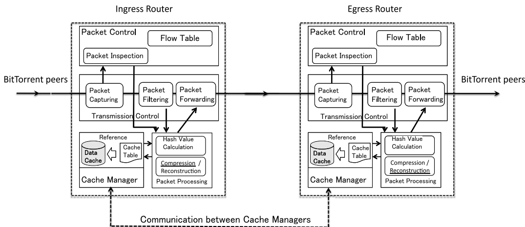
Fig. 2 Architecture overview.
