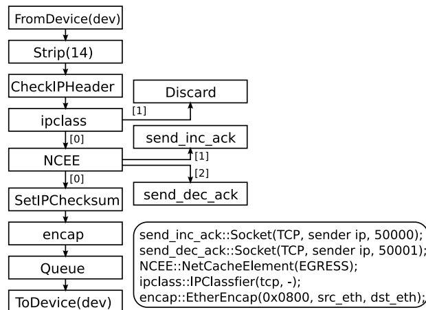
Fig. 6 Structure of egress router in the Click model.
