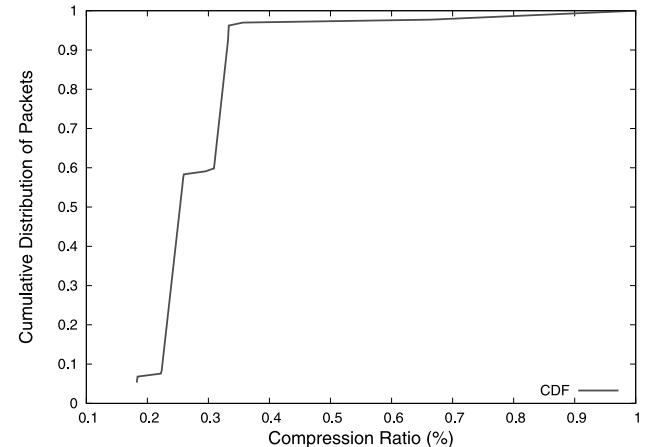
Fig. 11 Cumulative distribution of the traffic compression ratio (the second round).
