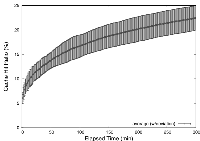
Fig. 14 Cumulative cache hit ratio averaged at every minute in the elapsed time for each 5-hour (300-minute) period.
