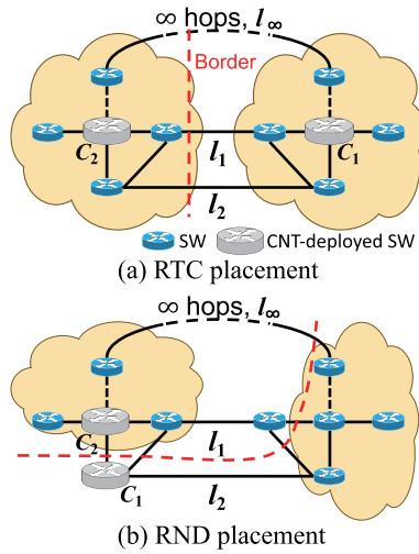
Fig. 8 Typical difference between RTC and RND placement.
