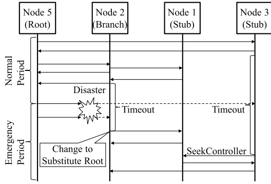
Fig. 10 Sequence of C-plane reconstruction when failure occurs.
