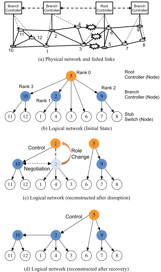
Fig. 9 C-plane reconstruction against network disruption and recovery.
