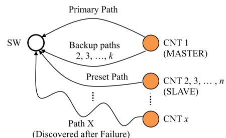
Fig. 1 Control path failover mechanisms. Backup paths: Path redundancy, CNT 2 to CNT n : Controller redundancy, Path X: Established after failure by reactive approach.
