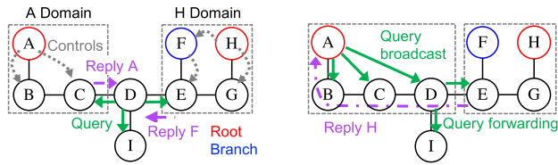
(a) Isolated node D discovers node A's domain. Node D sends queries to its adjacent nodes and it recognizes info of node A(F) from node C(E). (b) Node A finds adjacent domain dominated by node H. Node A broadcasts query to its children. Node D forwards the query to its neighbors. Node E replies info of Node H.
