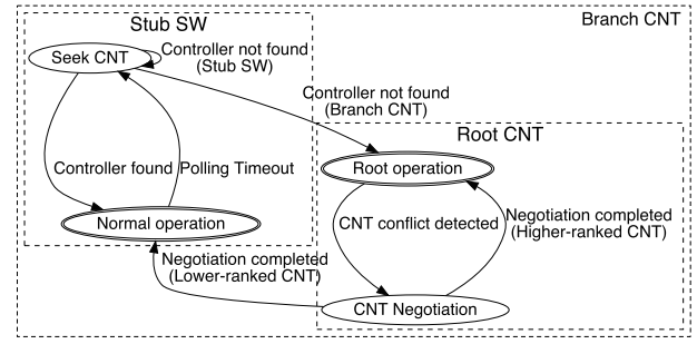
(a) State transition diagram for C-plane Reconstruction.
