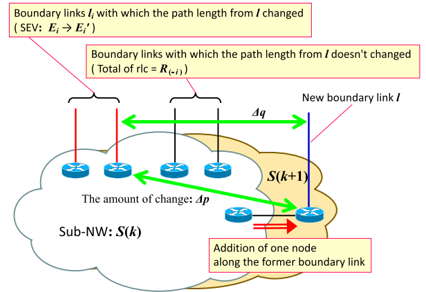
Fig. A-1 The relationship between boundary link pair in Sub-NW extension without increasing boundary link.
