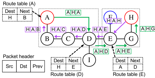
(c) Negotiation packet is sent via hop-by-hop forwarding for routing. The packet includes the previous node's information. Intermediate node E recognizes a route to source of the negotiation packet.
