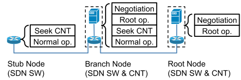
(b) Node architecture.
