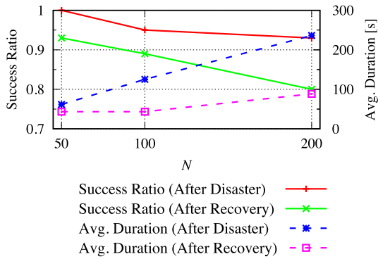
Fig. 13 Simulation results of C-plane reconstruction.
