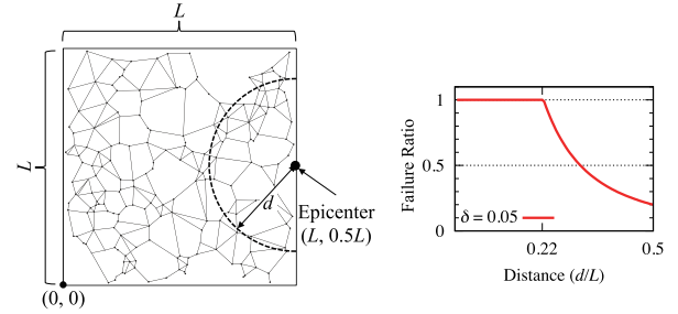
Fig. 6 Left: Seismic events. The epicenter is placed at eastside (L, 0.5L) following the Great East Japan Earthquake. Right: Relationship between distance from epicenter and failure ratio.
