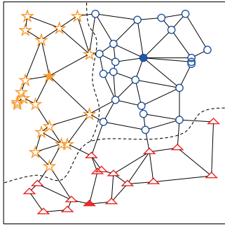
Fig. 5 An example of network separation via Algorithm 1 ( N = 60 ). The nodes having the same shape (color) belong to the same Sub-NW. The filled symbols denote the nodes that deploy controller functionality for their Sub-NWs. Star(orange), triangle(red), and circle(blue) Sub-NWs include 20, 17, and 23 nodes, respectively.
