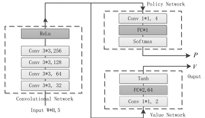
Fig. 3 Neural network structure.
