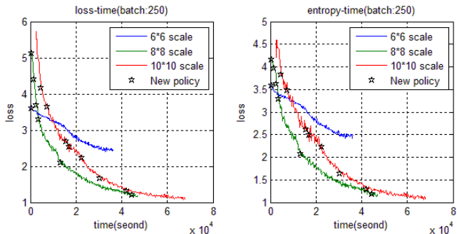
Fig. 5 Relationship between loss, entropy and training time.
