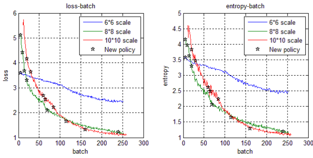
Fig. 4 Relationship between loss, entropy and training batch.
