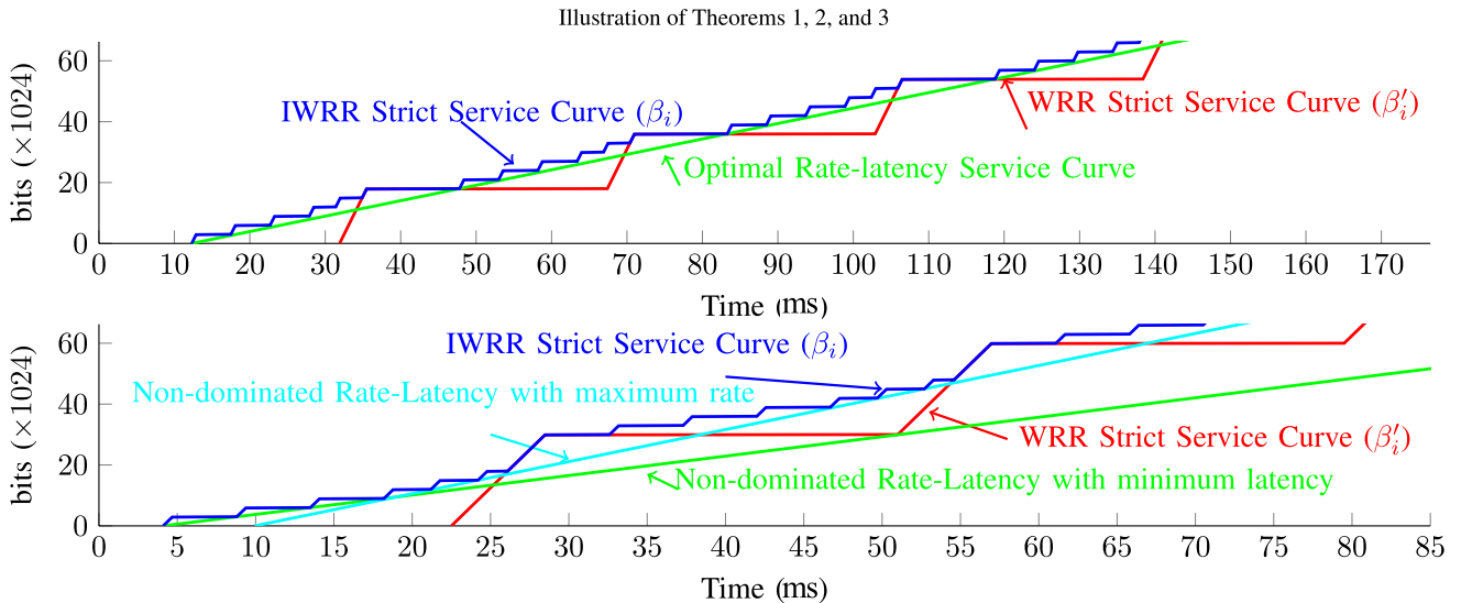
Fig. 3 Strict service curves obtained in Sect.5 for an example with four input flows, weights = \{4, 6, 7, 10\} , l_i^{\min} = \{4096, 3072, 4608, 3072\} bits, l_i^{\max} = \{8704, 5632, 6656, 8192\} bits and \beta(t) = ct with c = 10 Mb/s (i.e., the aggregate of all flows is served at a constant rate). The figure shows the IWRR service curve \beta_i and the WRR strict service curve \beta'_i for two of the flows; it also shows the non-dominated rate-latency strict service curves \beta_{r_0^*, T_0^*} and \beta_{r_k^*, T_k^*} of Theorem 3 (in the top panel both are equal).
