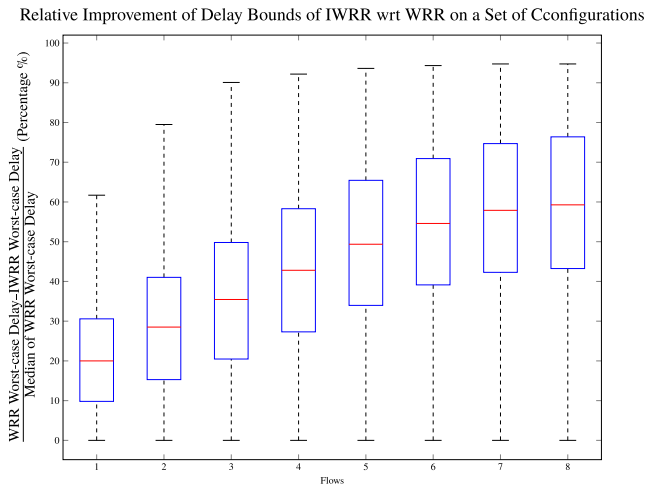
Fig. 5 Box-and-whisker plots of difference between WRR and IWRR delay bounds normalized to the median of WRR delay bounds, for several systems with weights picked uniformly at random in [10, 50] , assigned to flow by increasing order, and a packet length picked uniformly at random in [64, 1522] bytes.
