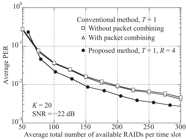
Fig. 6 Average PER as a function of average total number of available RAIDs per random access time slot.
