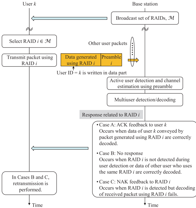
Fig. 1 Basic operational flow of random access with multi-packet reception.
