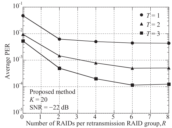
Fig. 4 Average PER as a function of the number of RAIDs per retransmission RAID group, R .
