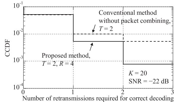
Fig. 8 CCDF of number of retransmissions required for correct decoding.
