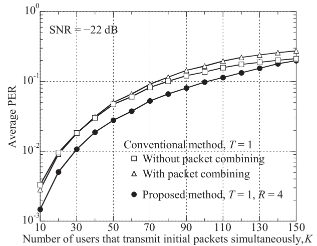
Fig. 7 Average PER as a function of number of users that transmit initial packets simultaneously, K .
