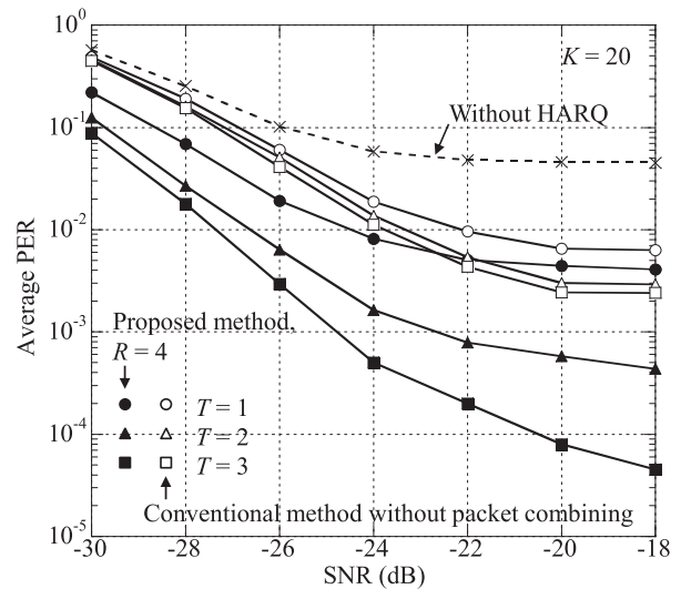
Fig. 5 Average PER as a function of SNR with maximum number of retransmissions, T , as a parameter.
