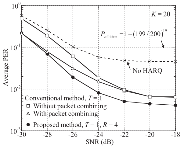
Fig. 3 Average PER as a function of SNR.
