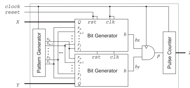
Fig. 4 Truncated multiplier based on bit-level processing.
