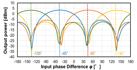
Fig. 5 Simulation results of on-chip Butler matrix.
