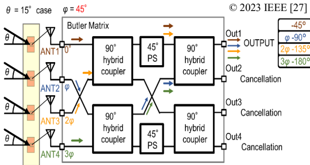
Fig. 3 On-chip butler matrix operation at input phase difference \varphi=45^\circ .
