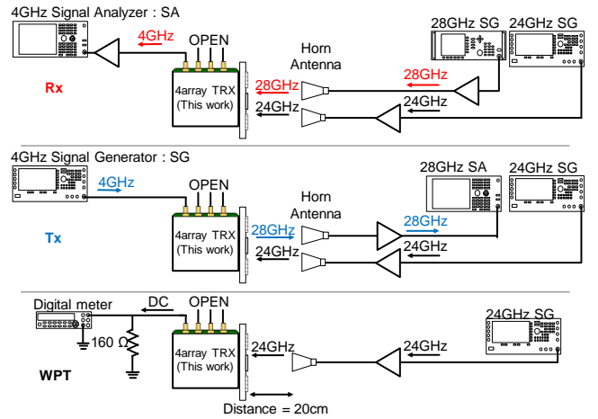
Fig. 12 OTA measurement setup of the relay transceiver.
