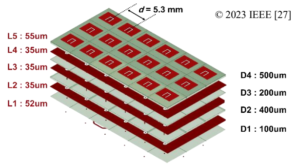
Fig. 9 Antenna model and layer illustration.
