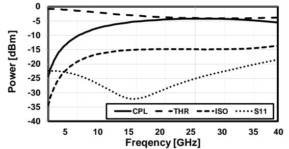
Fig.4 Simulation results of 90° hybrid coupler.
