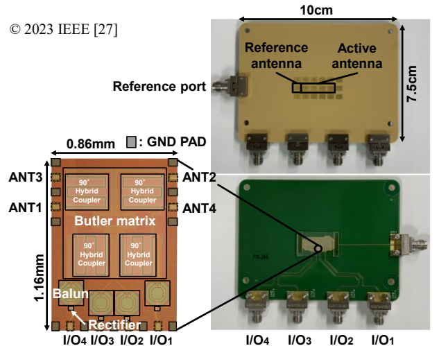
Fig. 10 Photo of proposed relay transceiver and chip micrograph.
