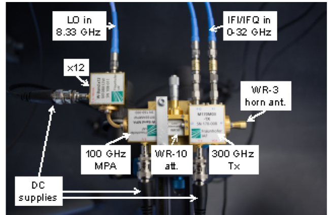
Fig. 14 Close-up of the transmitter module chain.
