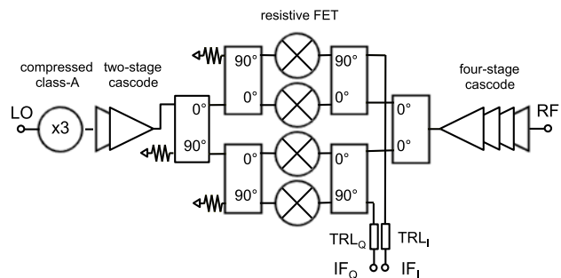
Fig. 4 Circuit architecture and chip photograph of the 300 GHz transmit MMIC. Chip size is 0.75 \times 3.25 \text{ mm}^2 .
