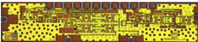
Fig. 4 Circuit architecture and chip photograph of the 300 GHz transmit MMIC. Chip size is 0.75 \times 3.25 \text{ mm}^2 .
