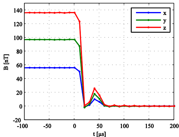
Fig. 8 System response of the LTS SQUID system to a 20 \mu s transient; samples at 10 \mu s intervals.
