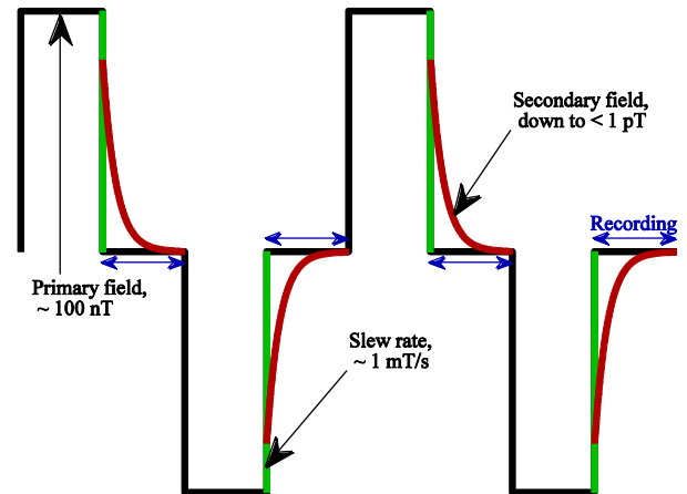
Fig. 2 Timing of TX signal (primary field) and the recorded transient response (secondary field) in a TEM measurement.
