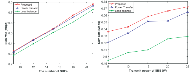
Fig. 2 Sum rate varies with the number of SUEs
