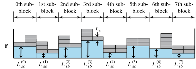
Fig. A.3 Example of received signals with interference light varying by sub-block ( p chips) and user sequences ( p = 2, q = 4 ).
