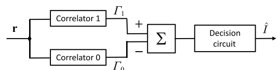
Fig. A-1 Block diagram of EWO decoder ( p = 2 ).
