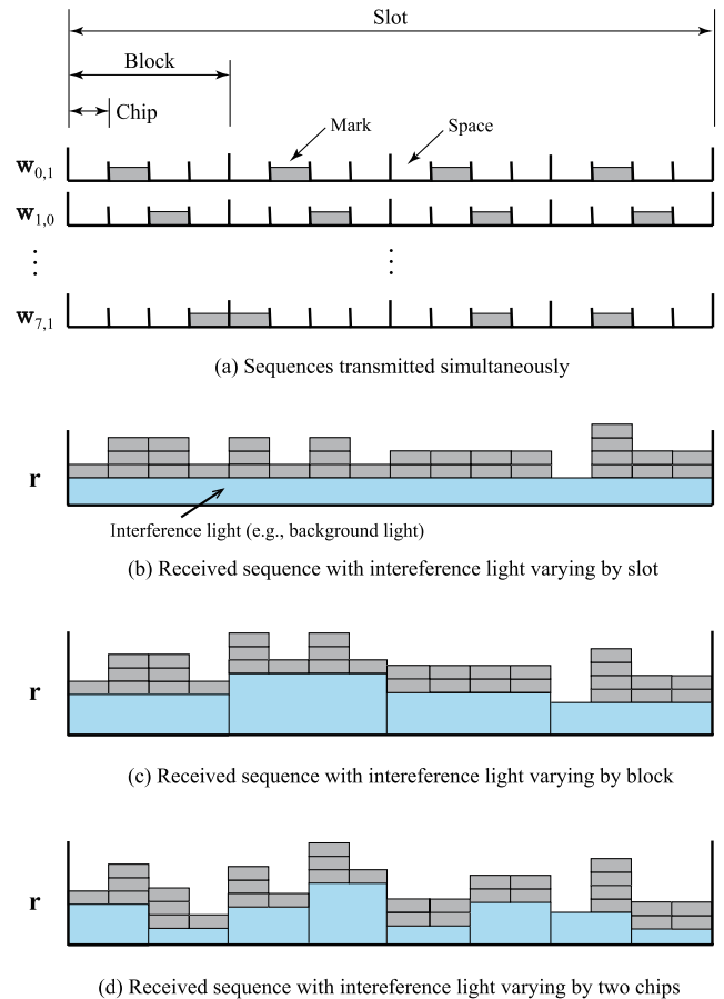
Fig. 1 Examples of multiplexed signals and interference light in optical CDMA system using GMPSC and the EWO scheme.
