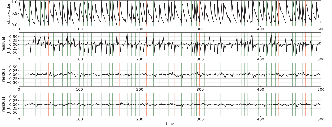
Fig. 1 Example of experimental results. The top figure shows a time series of observations for the degradation recovery process. The other figures show the residuals between the ground truth and the predictions by (second) the vanilla LSTM, (third) the reinitialization method, and (bottom) the concatenation method, respectively.
