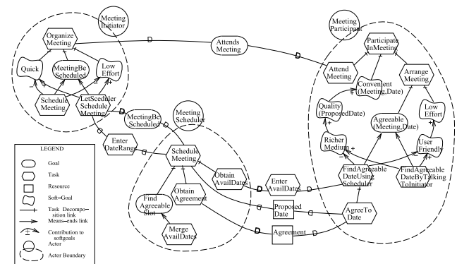
Fig. 13 iStar model in [1]
