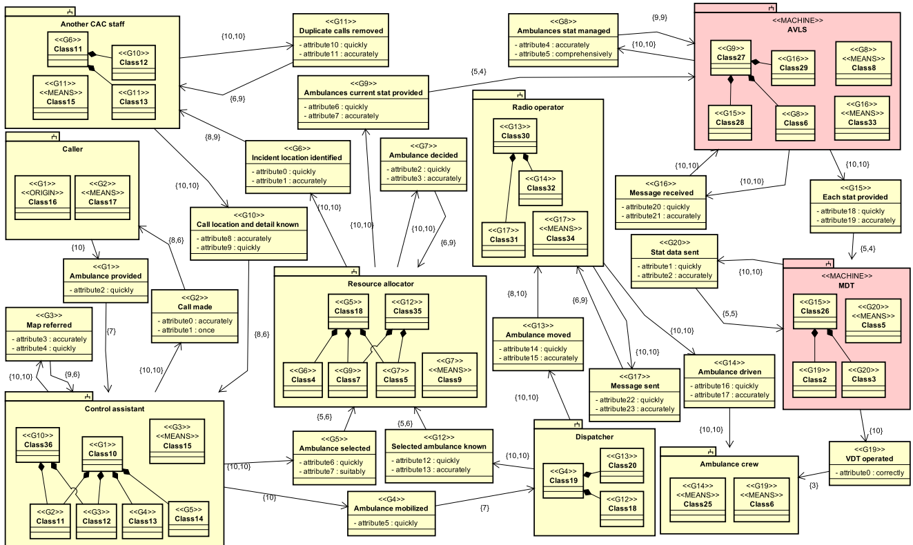
Fig. 12 To-be model of the ambulances dispatch
