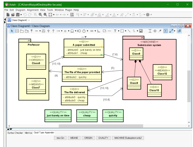
Fig. 6 Snapshot of Editor
