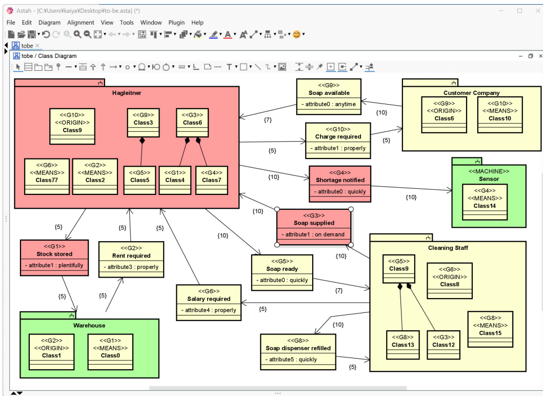
Fig. 10 To-be model of the stock management in Hagleitner, with the result of delegation tracer
