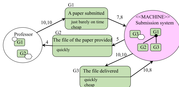
Fig. 2 To-be model of submitting a paper written in the iStar-based notation
