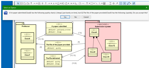
Fig. 8 Quality tracer
