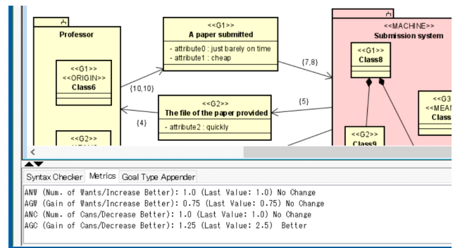
Fig. 7 Metrics calculator
