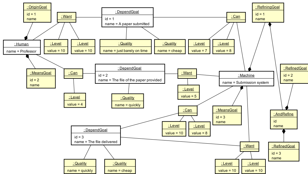
Fig. 4 Model corresponding to the to-be model in Fig. 2 written in the meta-model-based notation (i.e. an instance of the meta-model in Fig. 3)
