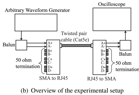
Fig. 6 Experimental setup using Cat5e cable.
