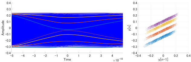
(c) Closed eye diagram and corresponding 2D mapping
