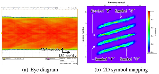
Fig. 11 Experimental result of 2D symbol mapping using that of the received symbol at 4 Gbps PAM-4 on the 1 m-long MSL.
