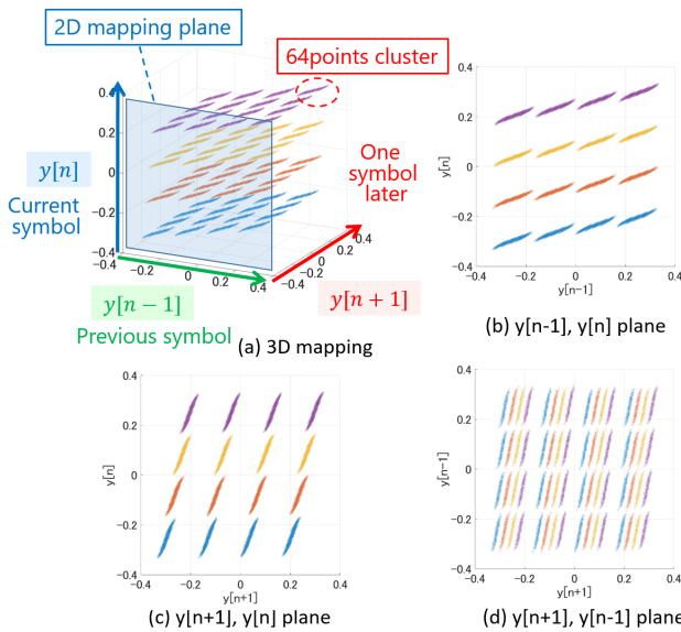
Fig. 12 Simulation results of 3D mapping and views from various planes.
