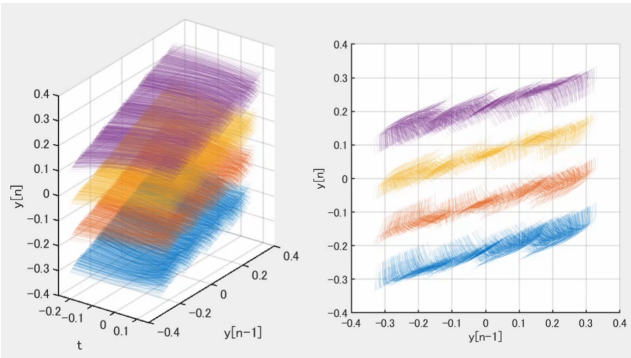
Fig. 15 Temporal superimposition of 2D mapping simulation results within a restricted time range.
