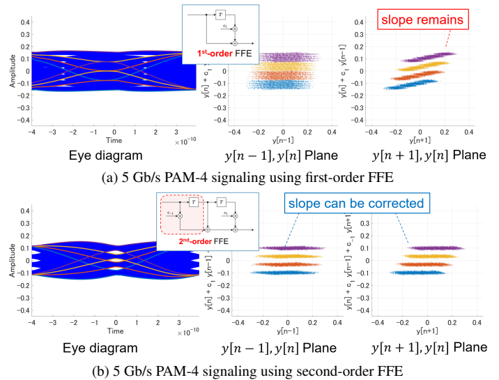
Fig. 13 Visualization of the waveform-shaping effect of the second-order FFE by 3D mapping.
