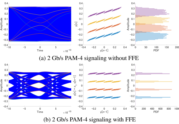
Fig. 6 Visualization of the equalizer effect (first-order equalization is a sufficient condition).
