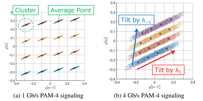
Fig. 3 Relationship between the distribution of symbol clusters and the impulse response coefficients for 2D mapping.
