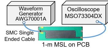
Fig. 10 Experimental setup.
