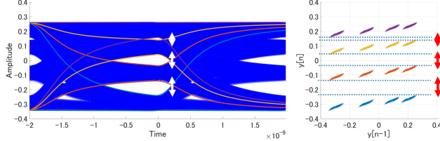
(b) Eye diagram and corresponding 2D mapping
