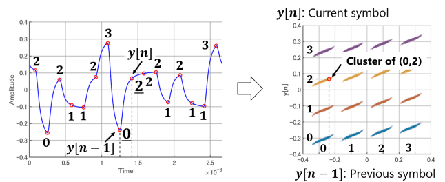
Fig. 1 2D mapping of the PAM-4 received symbols.
