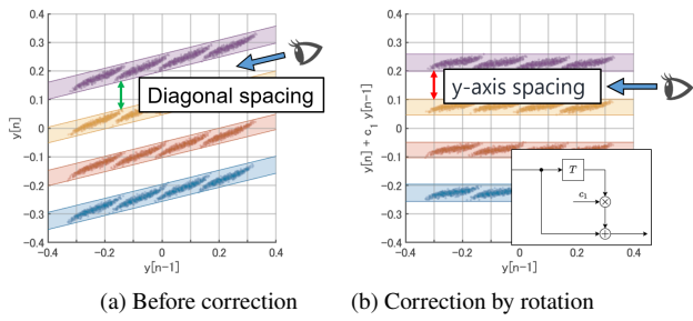
Fig. 5 Correlation between the 2D mapping tilt adjustment and the FFE functionality.
