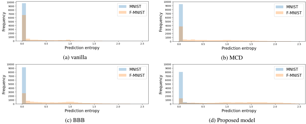
Fig. 3: Histograms of prediction entropy for each BNN method with MLP. The blue and orange bins correspond to the MNIST and Fashion-MNIST datasets, respectively; each dataset comprise 10,000 images. Each method concentrates on the low and high entropy regions for the MNIST and Fashion-MNIST datasets, respectively.
