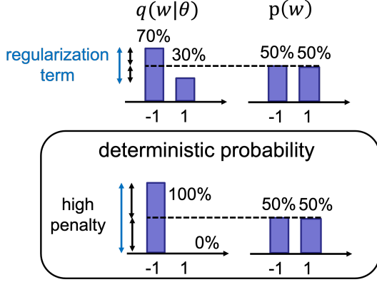
Fig. 2: Graphical overview of the regularization term which is a measure of the distance between the parameterized Bernoulli distribution q(w|\theta) and the Bernoulli distribution with 50%, p(w) . This regularization term strongly penalizes the Bernoulli distribution with deterministic probabilities.
