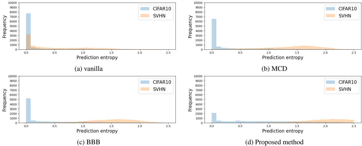
Fig. 4: Histograms of prediction entropy for each BNN method with ResNet-18. The blue and orange bins correspond to the CIFAR-10 and SVHN datasets, respectively; each dataset comprises 10,000 images. Our proposed method exhibits high prediction entropy on the out-of-distribution SVHN dataset compared to the other methods. Simultaneously, it demonstrates relatively high prediction entropy on the in-distribution CIFAR-10 dataset.
