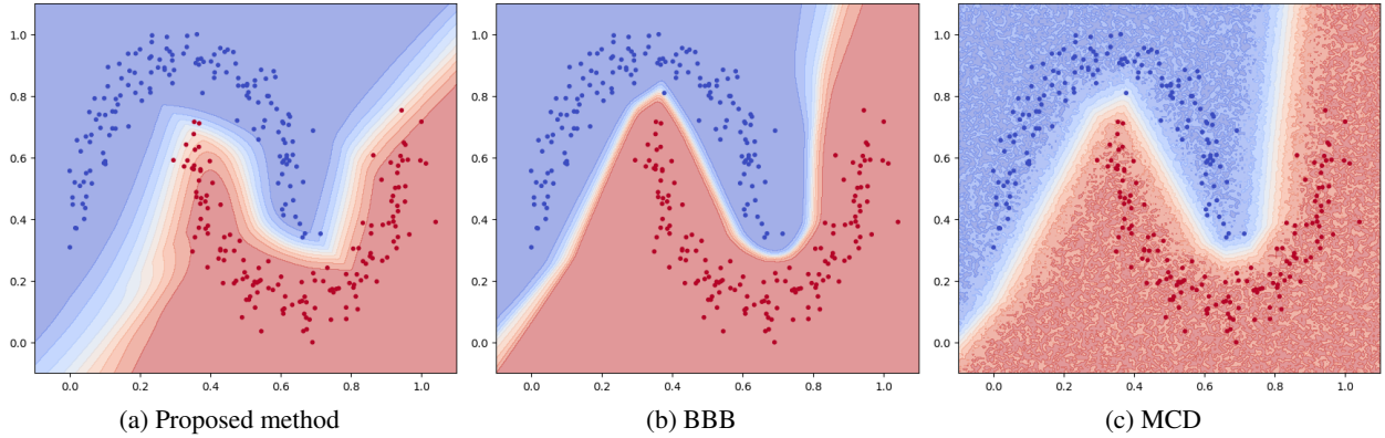
Fig. 5: Classification results on the two moons dataset with the three BNN methods. Left: proposed method; middle: BBB using the Gaussian distribution; right: MCD. Each result is the average of 10 prediction samples. The red and blue points represent class 0 and 1 data points, respectively. The model becomes more confident in classifying data as class 0 and 1 as the region becomes red and blue, respectively.
