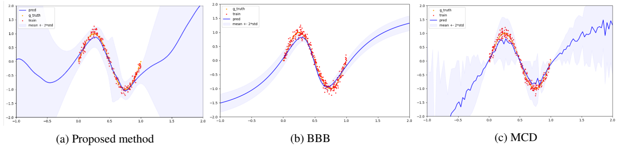
Fig. 6: Regression results with sine function for the three different BNN methods. Left: proposed algorithm; middle: BBB; right: MCD. The red data points represent the training data for the sine function, yellow line represents the true sine function, and blue line represents model predictions, which is the average of 10 sampled predictions. The light blue envelope represents the 95% confidence interval.
