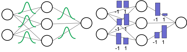
Fig. 1: Graphical overview of the difference in weights of BBB (left) and proposed method (right). The BBB’s weight is a Gaussian distribution, whereas that of the proposed method is a Bernoulli distribution. Binary weight values are represented as a Bernoulli distribution.
