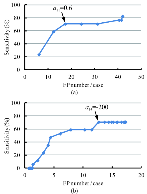
Fig. 9 FROC curves obtained by changing parameters of FP reduction process. FROC curves with parameters: (a) R_1 = 1.4, R_2 = 1.4, R_3 = 1.0, R_4 = 1.0, a_{11} = 0.2, \dots, 10.0, a_{14} = -500 and (b) R_1 = 1.4, R_2 = 1.4, R_3 = 1.0, R_4 = 1.0, a_{11} = 0.6, a_{14} = -500, \dots, 220 .
