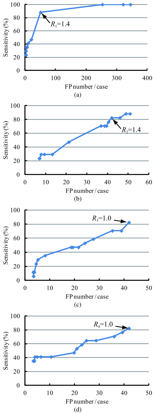
Fig. 8 FROC curves obtained by changing parameters of FP reduction process. FROC curves with parameters: (a) R_1 = 1.0, \dots, 9.0, R_2 = 1.0, R_3 = 1.0, R_4 = 1.0, a_{11} = 10.0, a_{14} = -500 , (b) R_1 = 1.4, R_2 = 1.0, \dots, 17.0, R_3 = 1.0, R_4 = 1.0, a_{11} = 10.0, a_{14} = -500 , (c) R_1 = 1.4, R_2 = 1.4, R_3 = 1.0, \dots, 17.0, R_4 = 1.0, a_{11} = 10.0, a_{14} = -500 , and (d) R_1 = 1.4, R_2 = 1.4, R_3 = 1.0, R_4 = 1.0, \dots, 17.0, a_{11} = 10.0, a_{14} = -500 .
