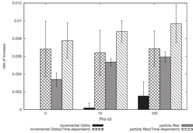
Fig. 10 Prediction performance of time-dependent inference methods. Error bars represent one sample standard deviation.
