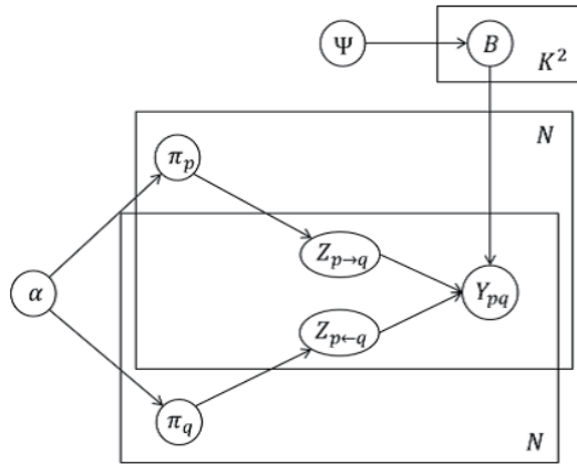
Fig. 1 Graphical model of MMSB.
