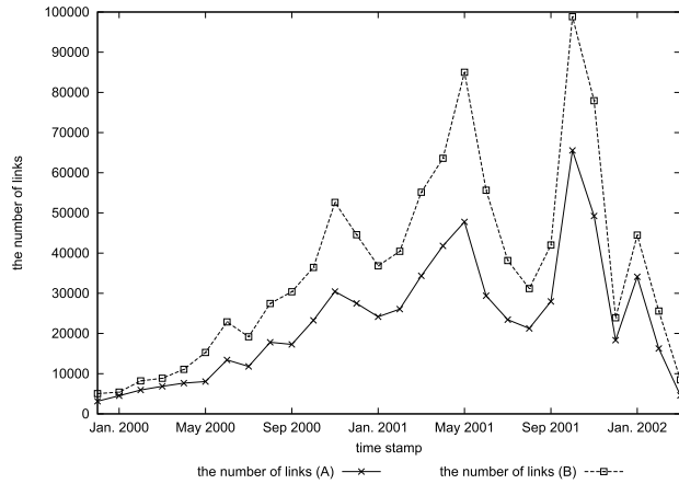
Fig. 7 The number of links at each time interval.
