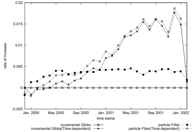
Fig. 11 Prediction performance of time-dependent inference methods (with Dataset A when |R(p, q)| = 0 ) in time series plots.
