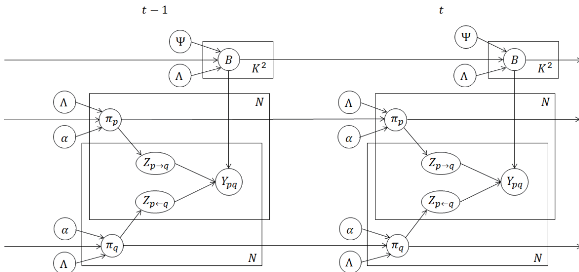
Fig. 6 Graphical model of time-dependent MMSB.
