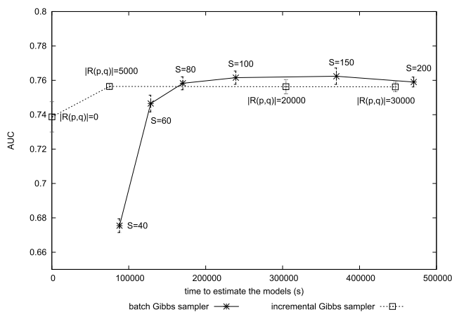
Fig. 9 Comparison of batch Gibbs sampler and incremental Gibbs sampler in terms of AUC. Error bars represent one sample standard deviation.
