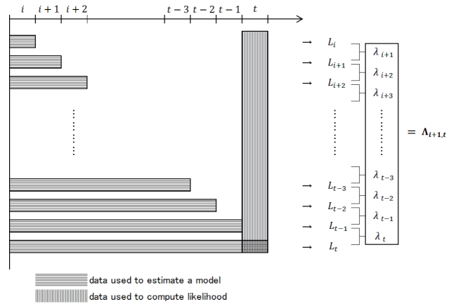
Fig. 5 Illustration of how to estimate \Lambda .
