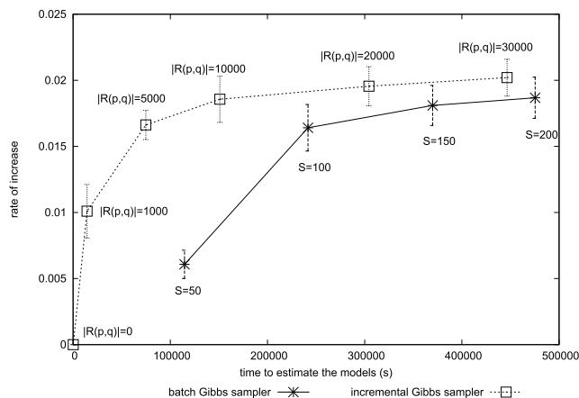
Fig. 8 Comparison of batch Gibbs sampler and incremental Gibbs sampler in terms of rate of increase of test-set log-likelihood. Error bars represent one sample standard deviation.
